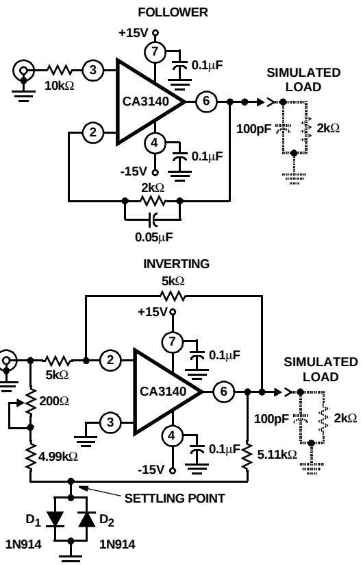
FIGURE 5B. TEST CIRCUITS
