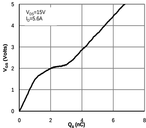
Figure 7: Gate-Charge Characteristics
