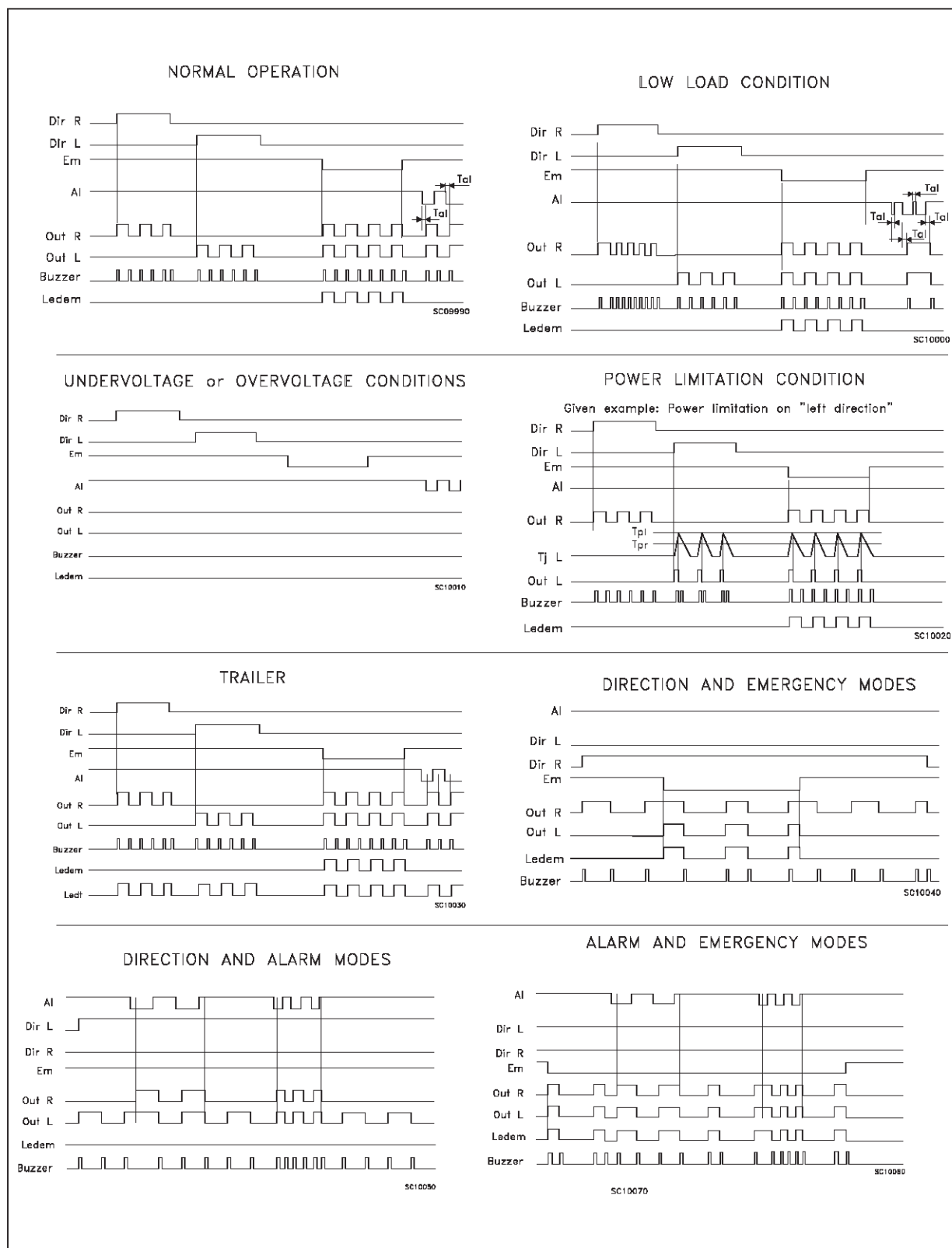
FIGURE 2: Switching Waveforms
