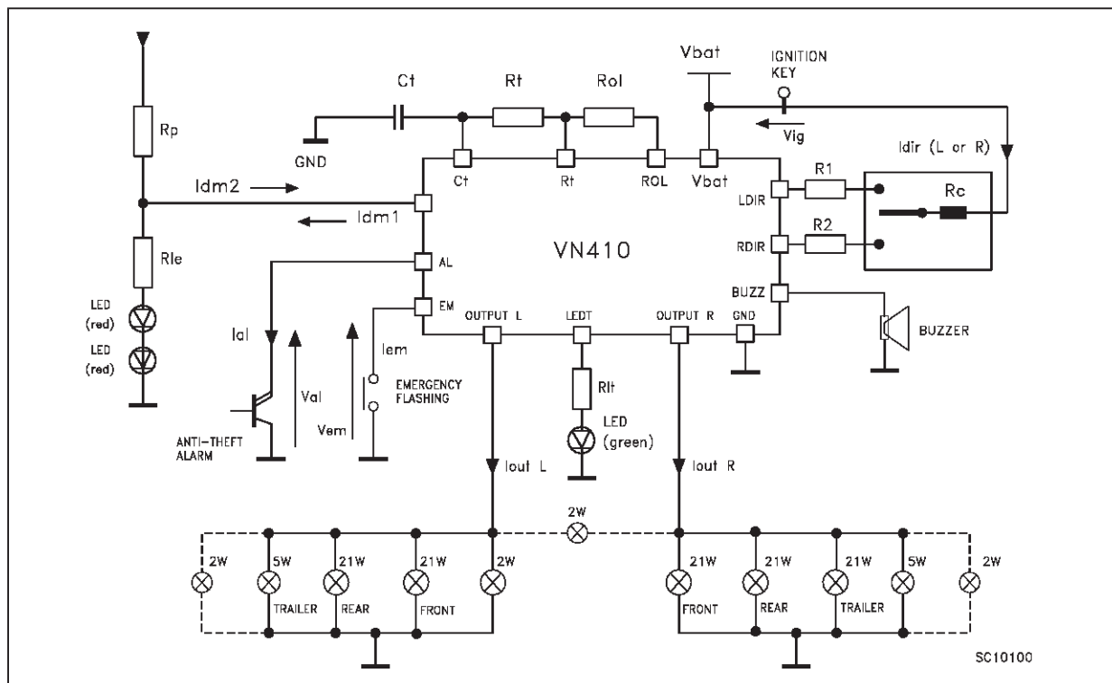
TYPICAL APPLICATION DIAGRAM
