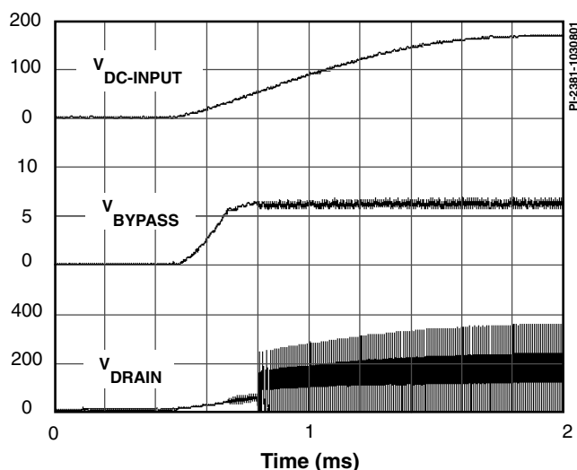
Figure 10. Power Up.
