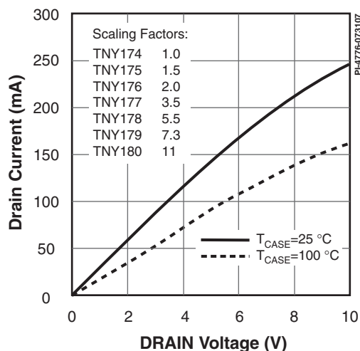
Figure 22. Output Characteristic.
