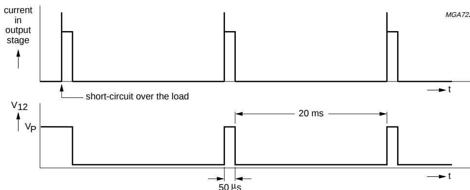
Fig.4 Short-circuit waveform.
