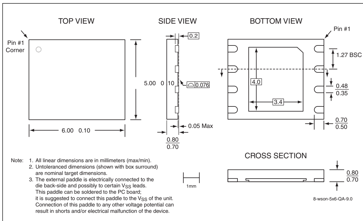
Figure 28: 8-Contact Very-very-thin, Small-outline, No-lead (WSN) SST Package Code: QA
