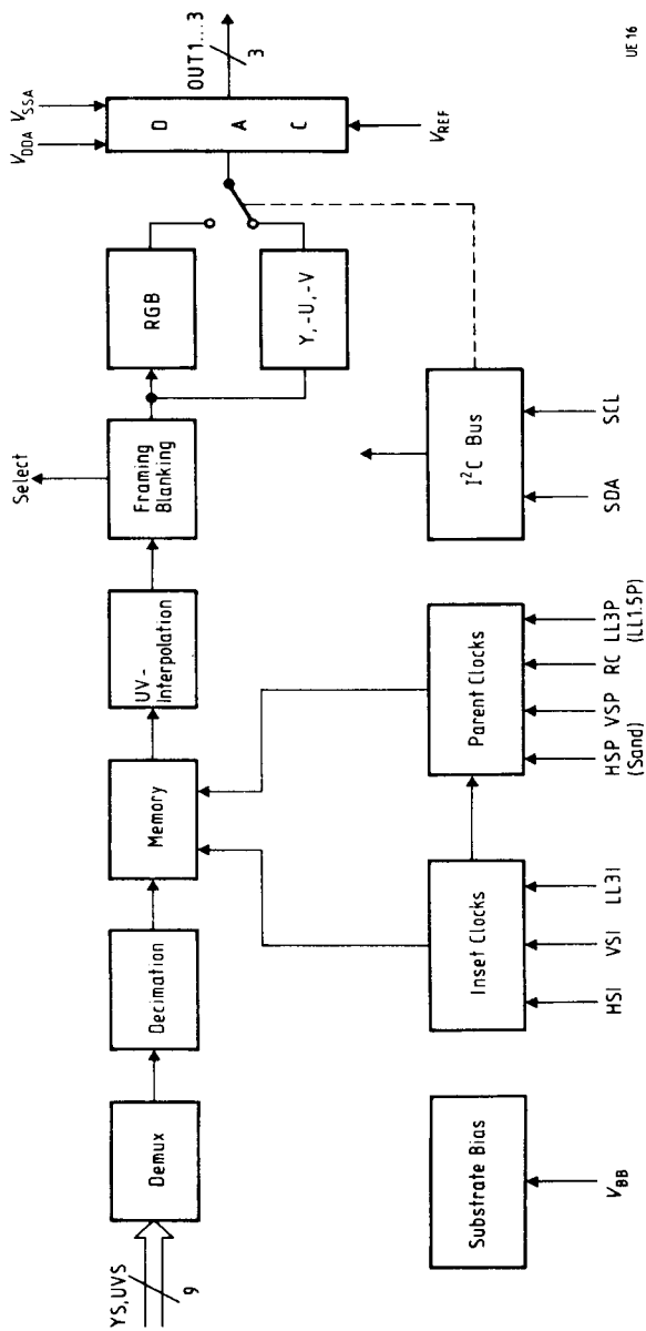
Block Diagram
