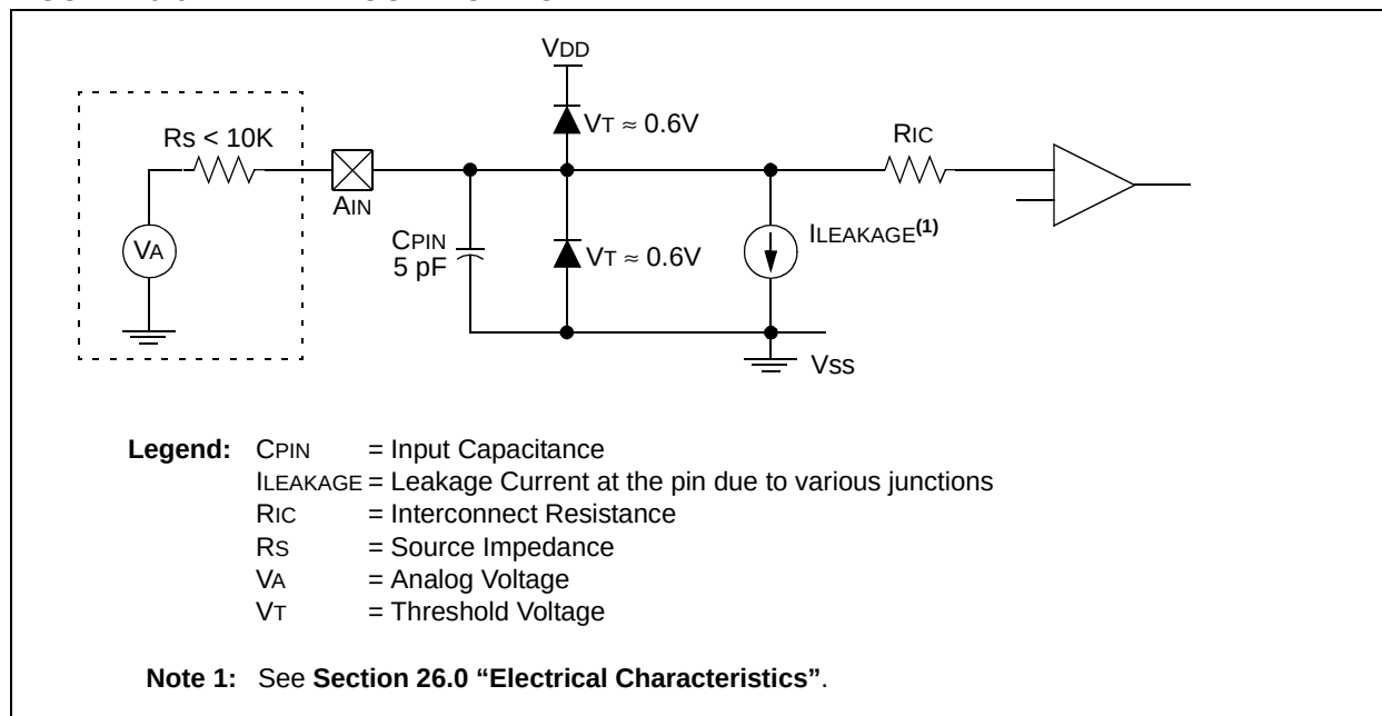
FIGURE 20-6: ANALOG INPUT MODEL
