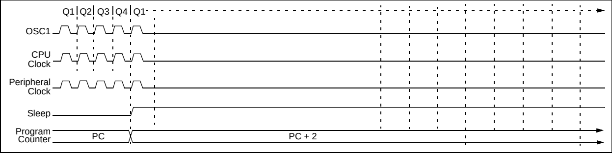
FIGURE 3-1: TRANSITION TIMING FOR ENTRY TO SLEEP MODE
