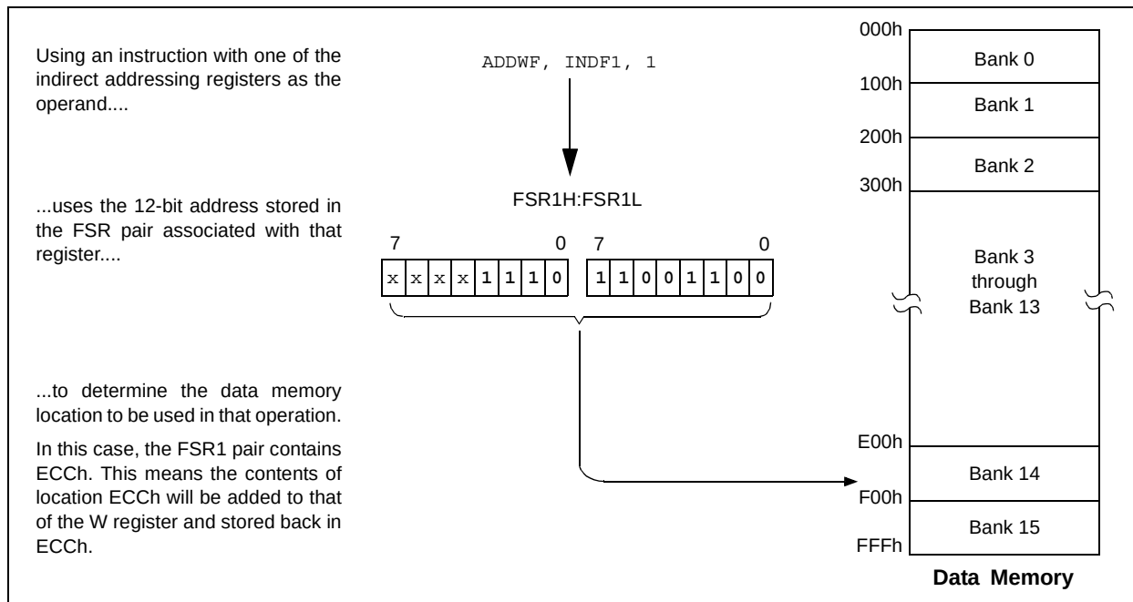
FIGURE 5-10: INDIRECT ADDRESSING
