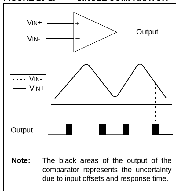
FIGURE 20-1: SINGLE COMPARATOR
