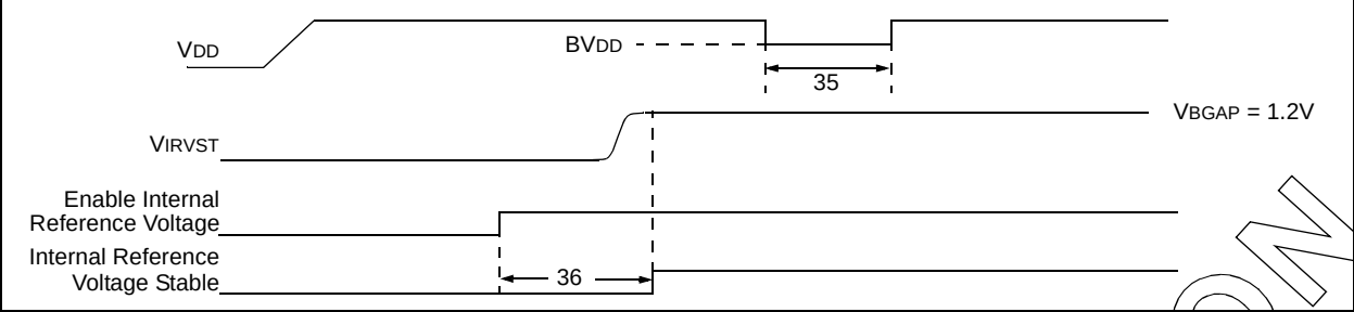
FIGURE 26-7: BROWN-OUT RESET TIMING
