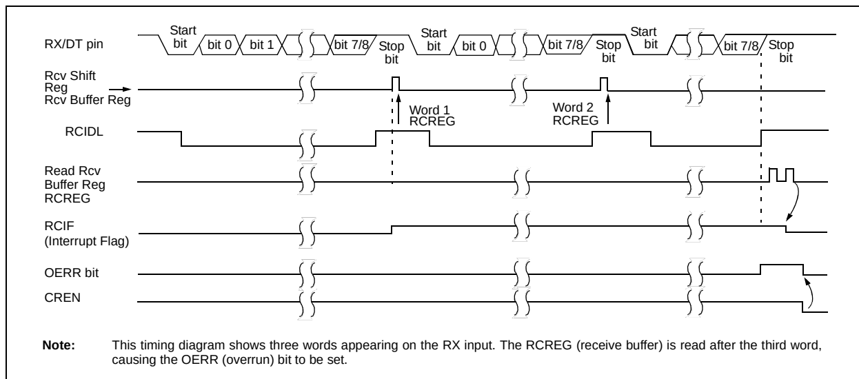
FIGURE 18-5: ASYNCHRONOUS RECEPTION
