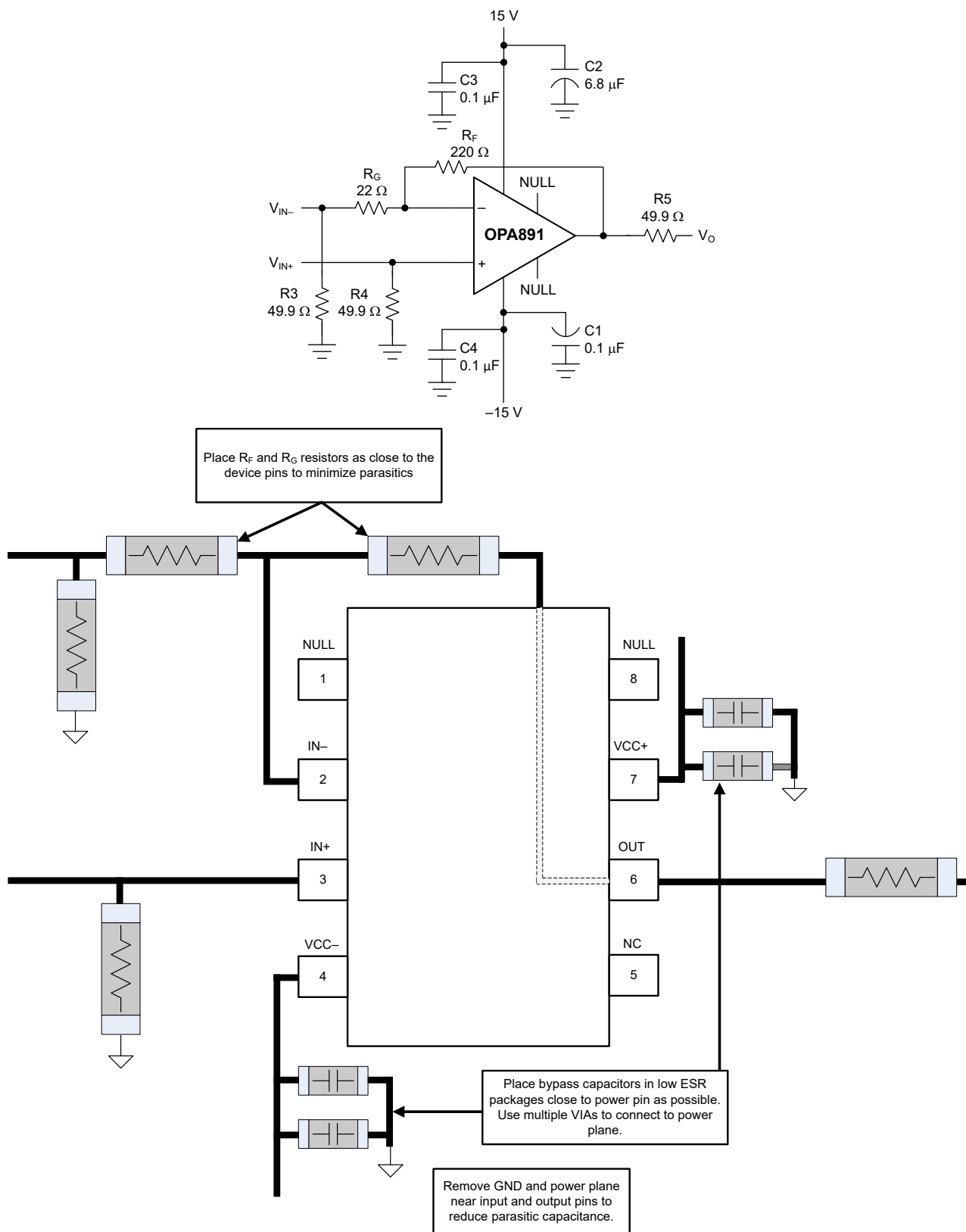
Figure 7-11. Layout Recommendations
