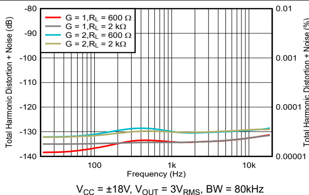
Figure 5-35. THD+N vs Frequency
