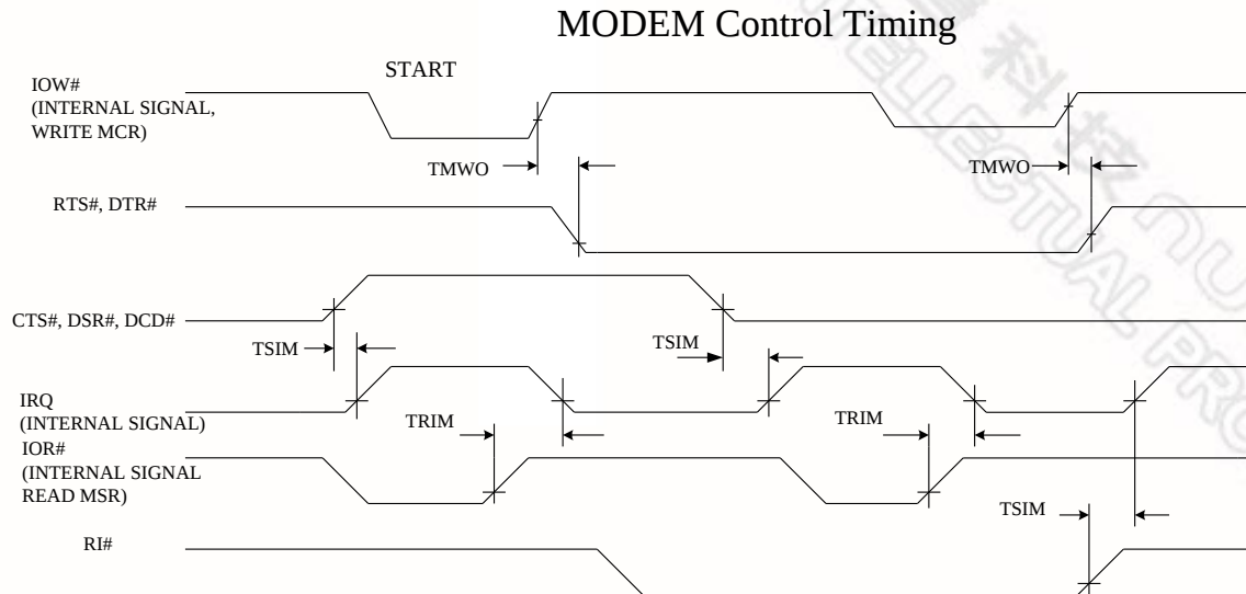
Modem Control Timing
