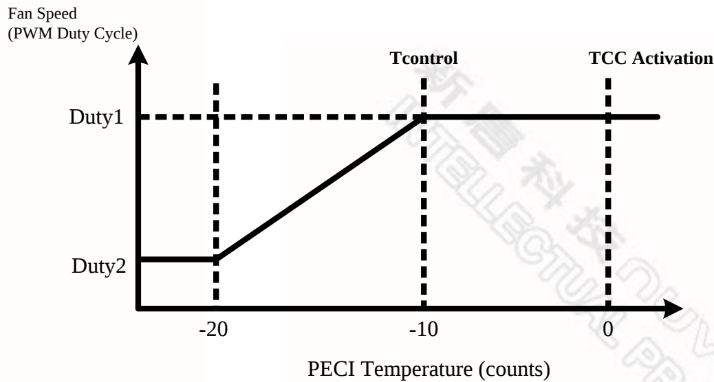
Figure 8-8 PECTemperature
