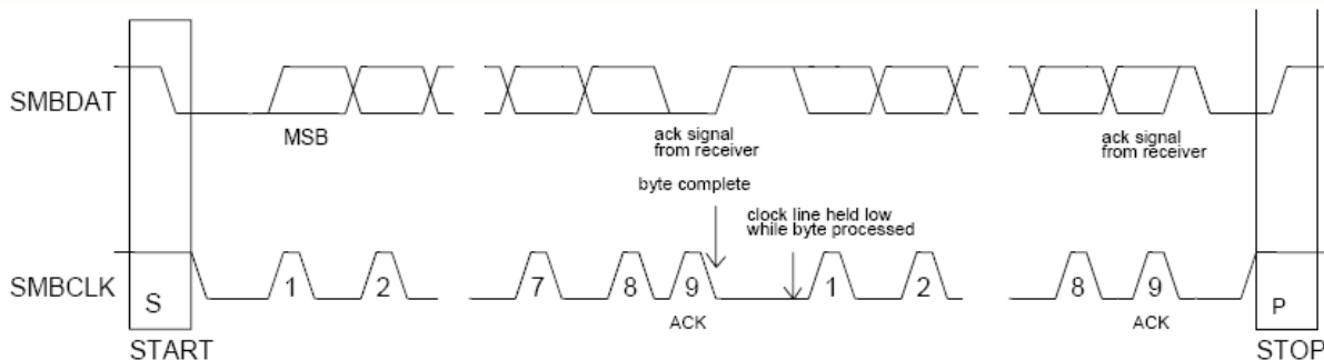
Figure 20-1 Data Transfer Format
