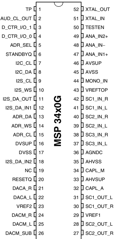
Fig. 4–7: PSDIP52-1/-2 package
