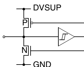
Fig. 4-18: Input/Output Pins: I2S_CL, I2S_WS, D_CTR_I/O_1, D_CTR_I/O_0
