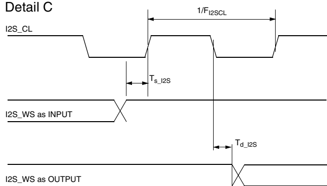
Fig. 4-27: I 2 S bus timing diagram
