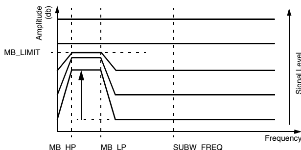
Fig. 2–6: Dynamic amplification
