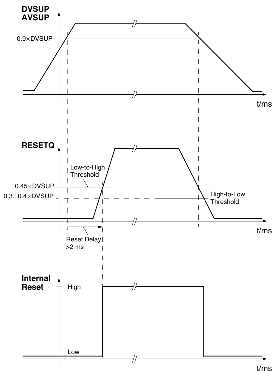
Fig. 4-25: Power-up sequence
