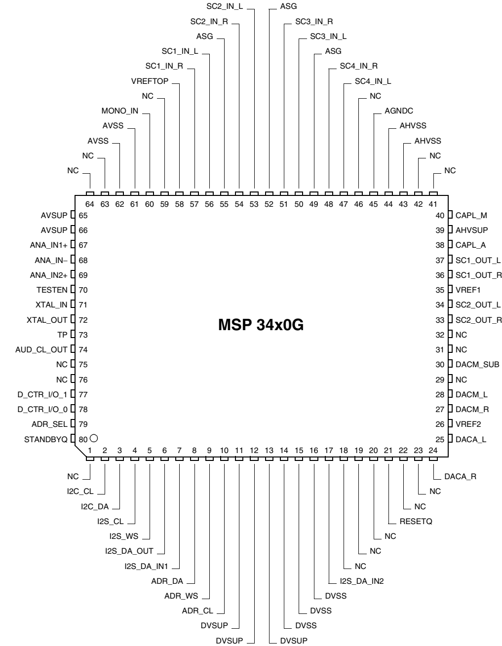
Fig. 4–8: PMQFP80-11 package
