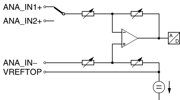
Fig. 4-15: Input Pins: VREFTOP, ANA_IN1+, ANA_IN-, ANA_IN2+
