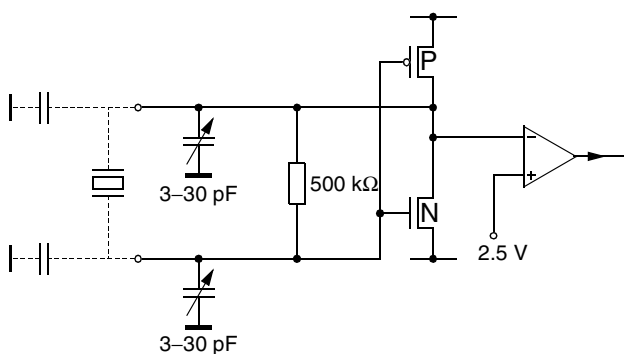
Fig. 4-19: Input/Output Pins: XTAL_IN, XTAL_OUT, AUD_CL_OUT
