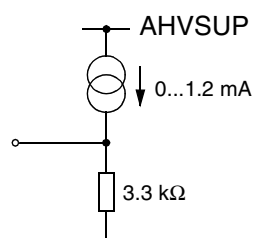
Fig. 4-20: Output Pins: DACA_R/L, DACM_R/L, DACM_SUB
