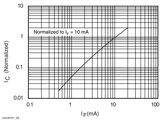
Fig. 2 - Collector Current vs. LED Forward Current
