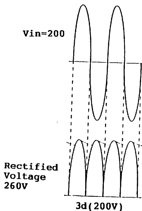
Full wave bridge rectification
