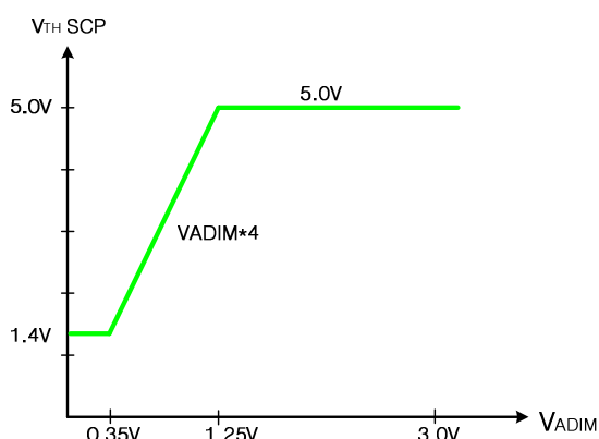
Fig 5. SCP threshold voltage based on ADIM voltage
