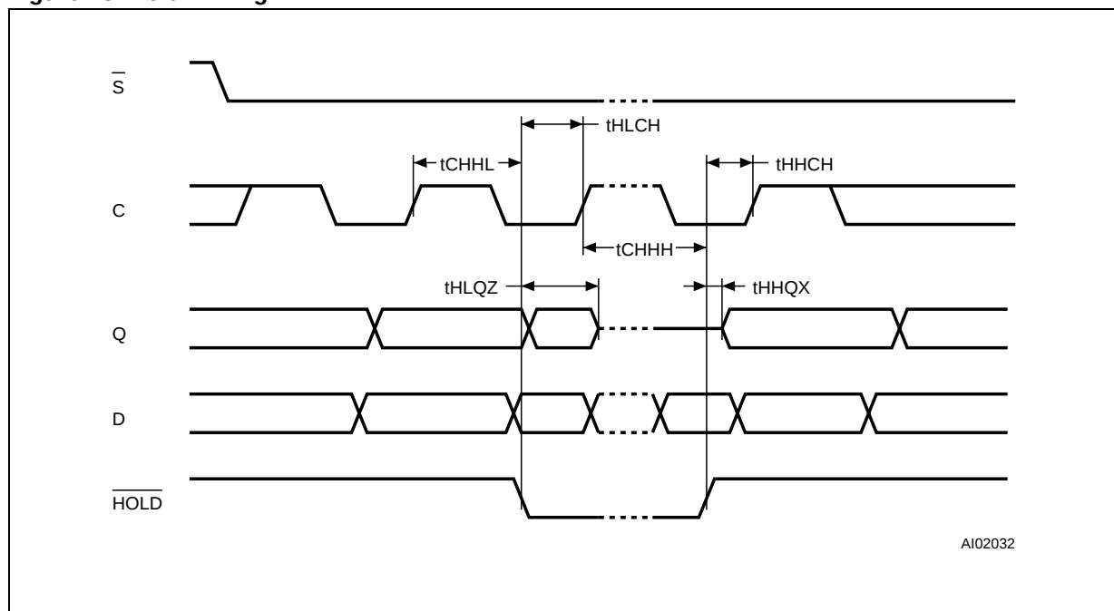
Figure 18. Hold Timing
