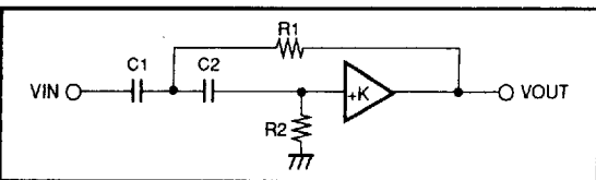
Fig.3 Positive feedback type secondary high pass filter circuit of bass boost block
