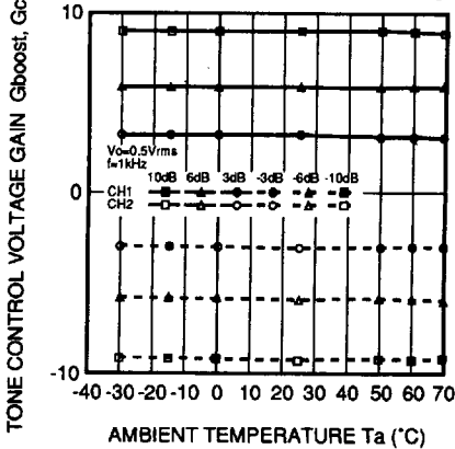
TONE CONTROL VOLTAGE GAIN (F3) VS. AMBIENT TEMPERATURE CHARACTERISTICS
