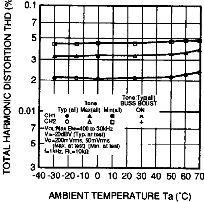
TOTAL HARMONIC DISTORTION (BUF OUT) VS. AMBIENT TEMPERATURE CHARACTERISTICS
