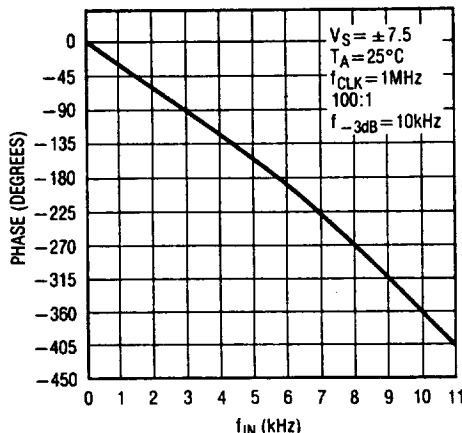
Graph 2. Phase Response
