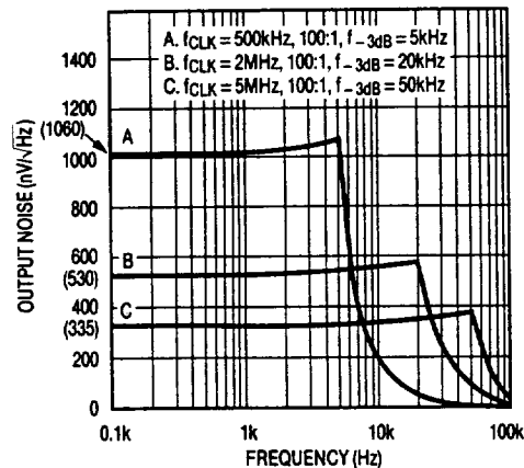
Graph 6. Noise Spectral Density
