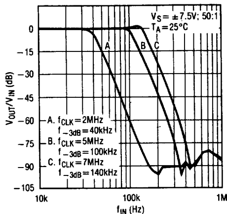
Graph 1. Amplitude Response
