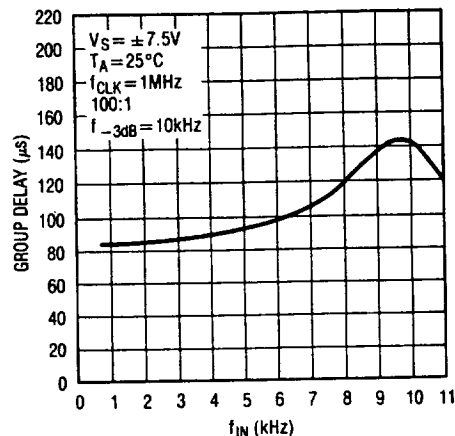
Graph 3. Group Delay vs Frequency
