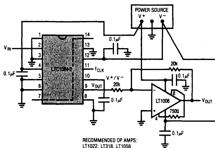
Figure 1. Buffering the Filter Output. The Buffer Op Amp Should Not Share the LTC1064-2 Power Lines.
