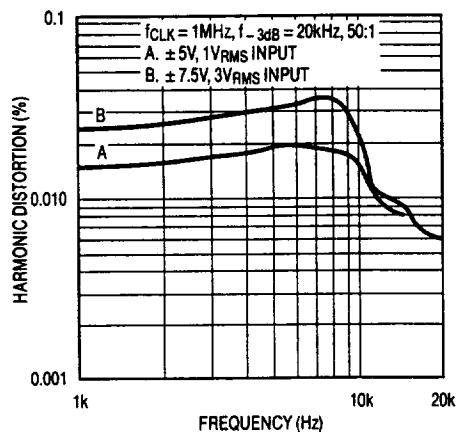
Graph 7. Harmonic Distortion vs Frequency
