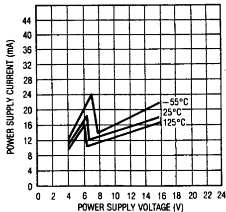
Graph 9. Power Supply vs Current
