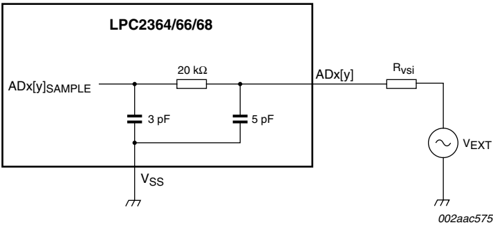
Fig 5. Suggested ADC interface - LPC2387 AD0[y] pin
