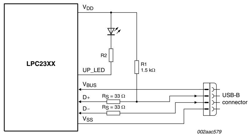
Fig 9. LPC2364/66/68 USB interface on a bus-powered device
