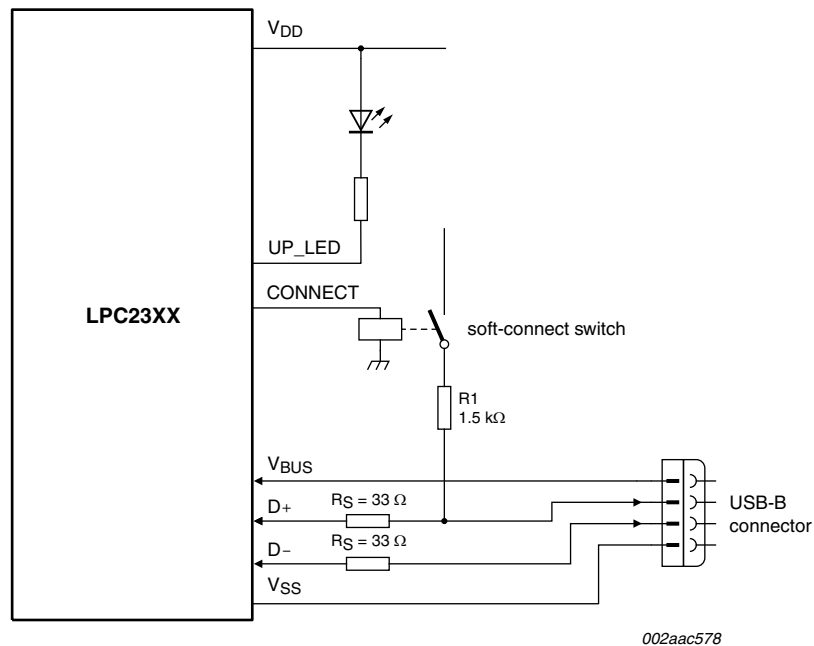
Fig 8. LPC2364/66/68 USB interface on a self-powered device
