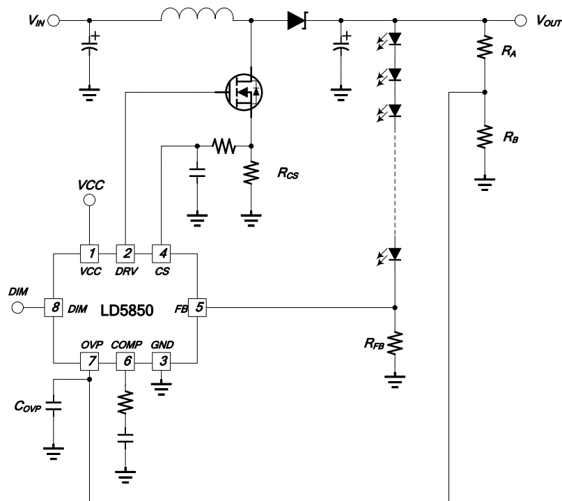
Fig. 1 Application circuit
