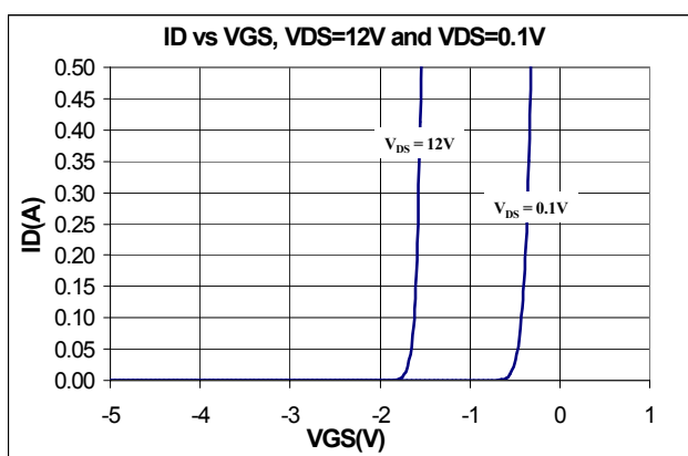
Figure 6 – Transfer Characteristic
