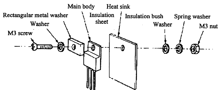
Fig.4 TO-220 system
