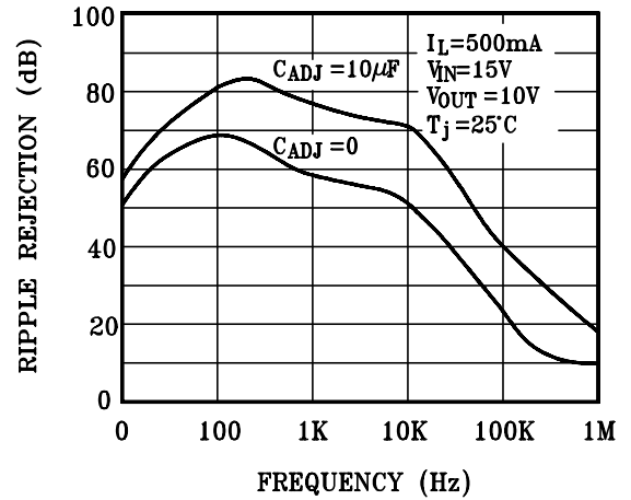
Ripple Rejection
