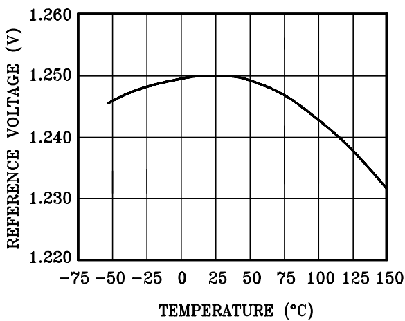
Temperature Stability
