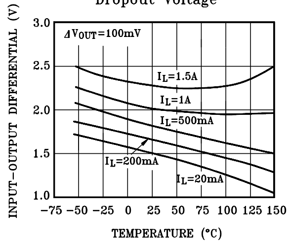
Dropout Voltage
