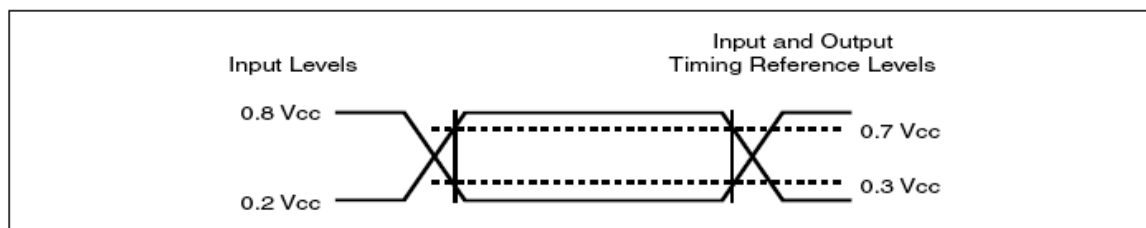
Figure 23. AC Measurement I/O Waveform
