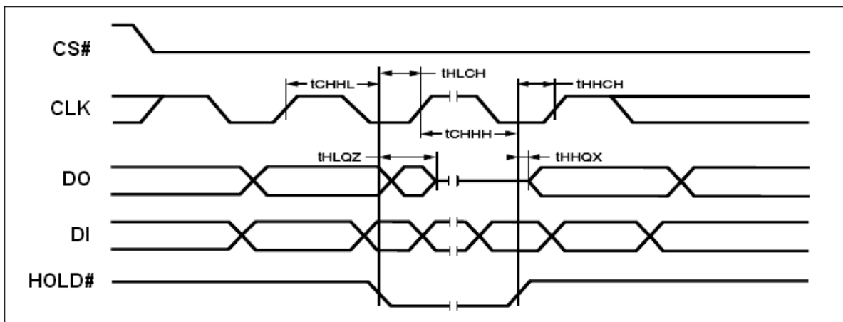
Figure 26. Hold Timing
