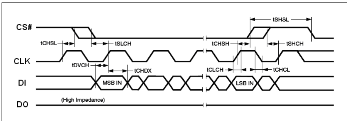
Figure 25. Input Timing
