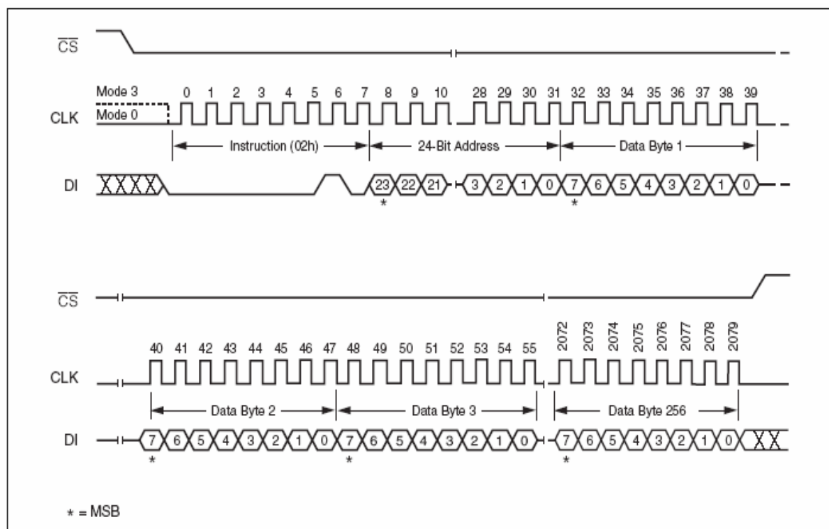
Figure 11. Page Program Instruction Sequence Diagram
