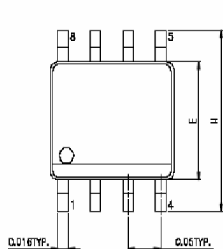
Figure 26. SOP 150 mil
