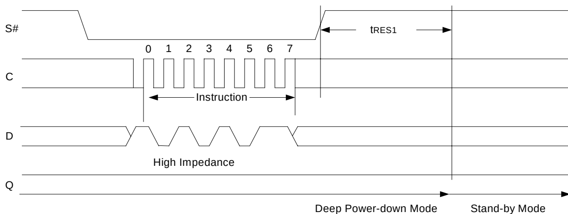
Figure 21: Release from Deep Power-down (RES) Sequence
