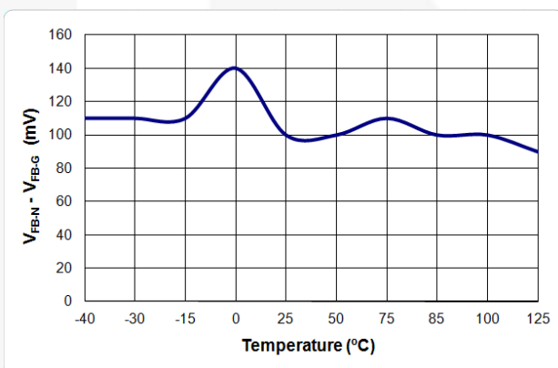
Figure 13. V_{FB-N} - V_{FB-G} vs. Temperature
