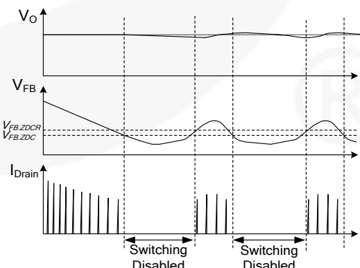
Figure 24. Burst-Mode Operation
