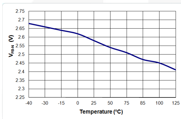
Figure 12. V_{FB-N} vs. Temperature
