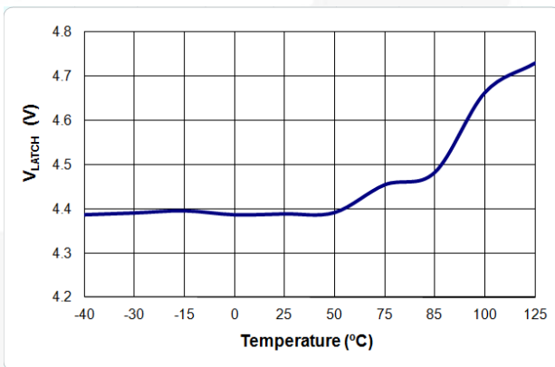
Figure 9. V LATCH vs. Temperature
