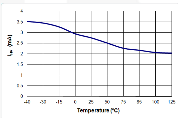
Figure 7. I HV vs. Temperature
