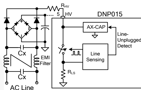
Figure 22. AX-CAP® Circuit
