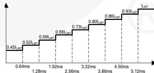
Figure 19. Current Limit Variation During Soft-Start
