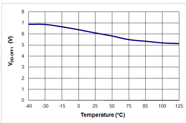
Figure 5. V DD-OFF1 vs. Temperature
