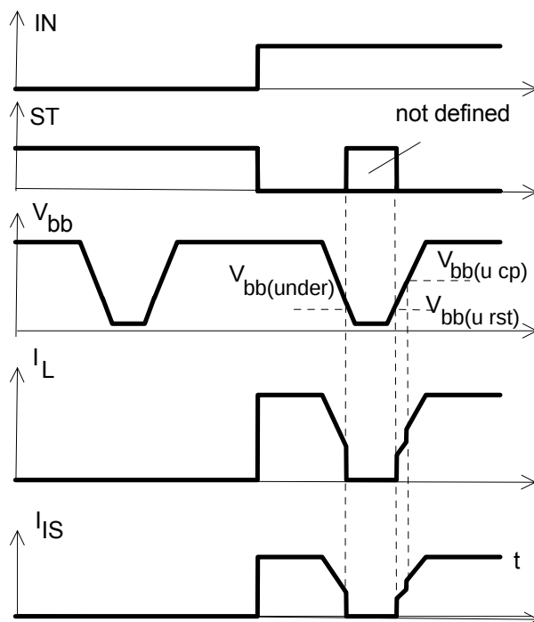
Figure 6a: Undervoltage:
