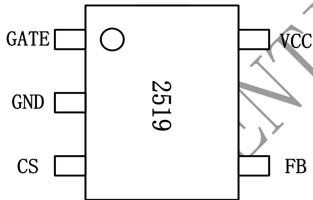
Fig2 Pin configuration
