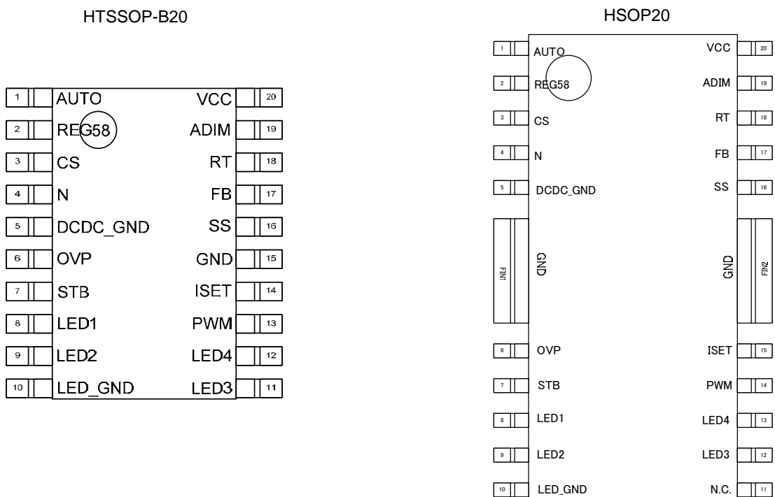
Figure 3. Pin Configuration
