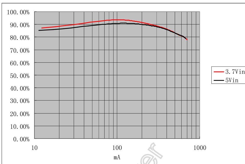
DC-DC3 2.5V Efficiency vs. Load
