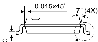
VIEW "A"
