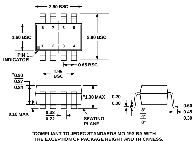
Figure 2. 8-Lead Thin Small Outline Transistor Package [TSOT] (UJ-8)
