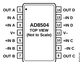
Figure 2. 14-Lead TSSOP (RU-14)
