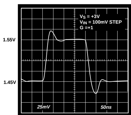
Figure 29. Pulse Response, V_S = +3\text{ V} , G = +1
